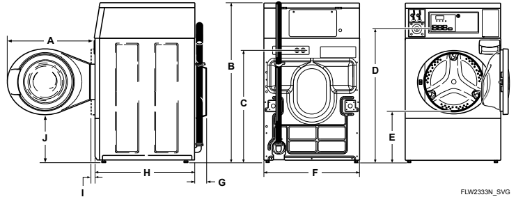
Models Equipped With Drain Hose
